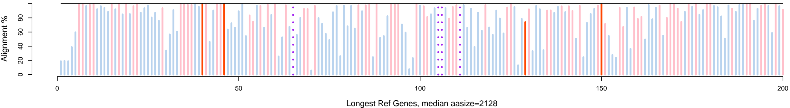
Gene set: dapplxjgiv11 (79% ref align, 38% best)
