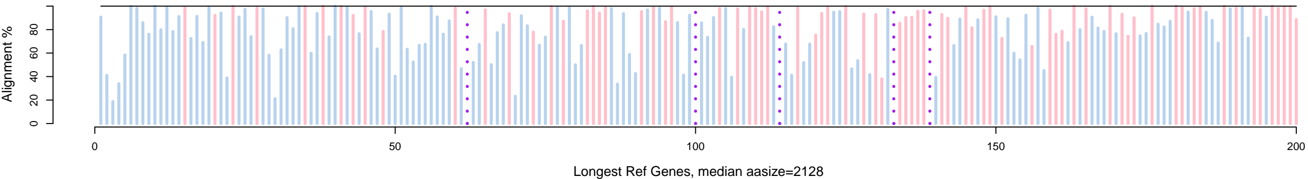
Gene set: dapmag (80% ref align, 37% best)
