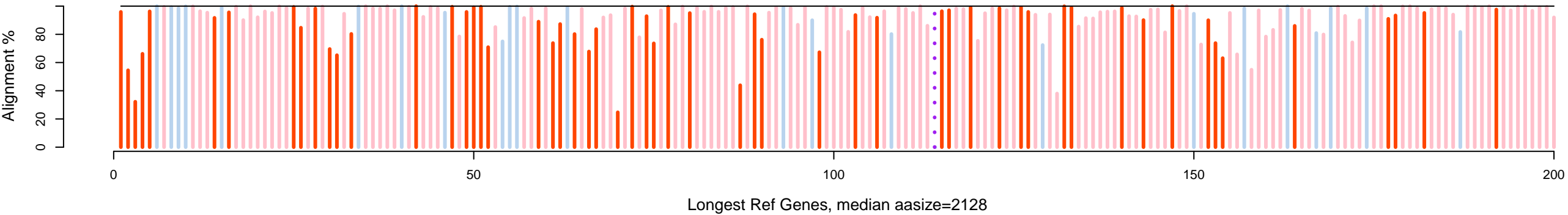
Gene set: dapmagevg14 (91% ref align, 88% best)
