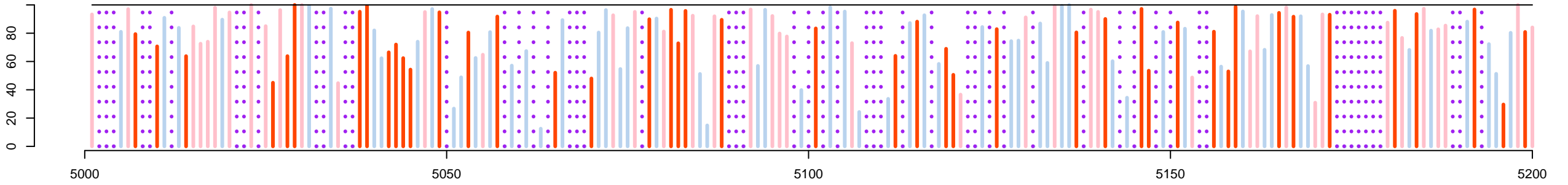
Gene set: tickxoevg14 (56% ref align, 43% best)
