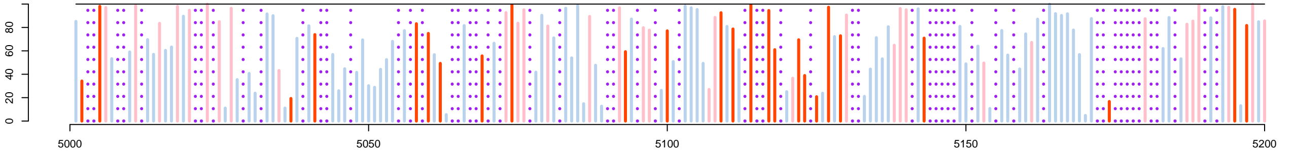
Gene set: tickixo (47% ref align, 29% best)
