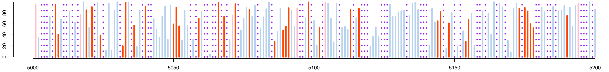
Gene set: ticktet (48% ref align, 21% best)
