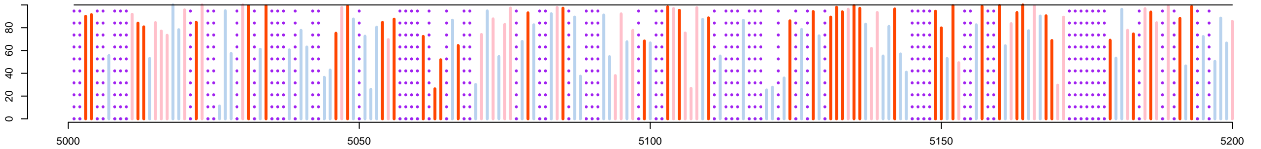
Gene set: tickzebevg13 (51% ref align, 38% best)
