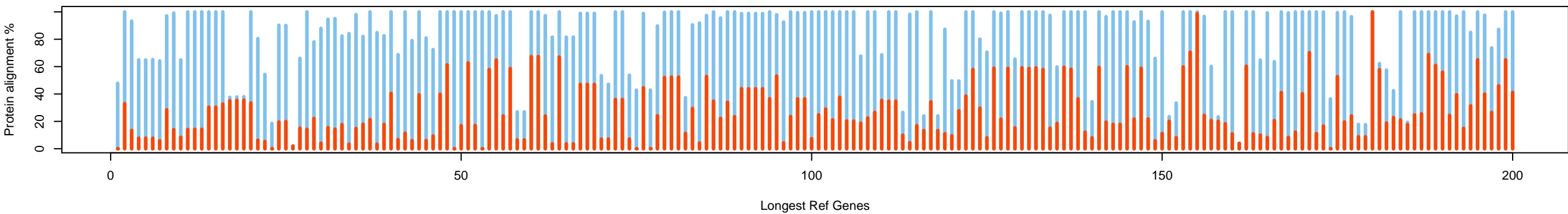
RefArath-plants: banana_tsa (28% ref)
