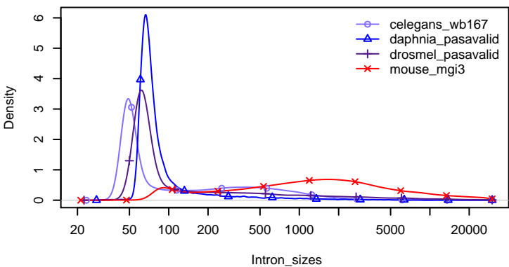
Eukaryote Intron_sizes
