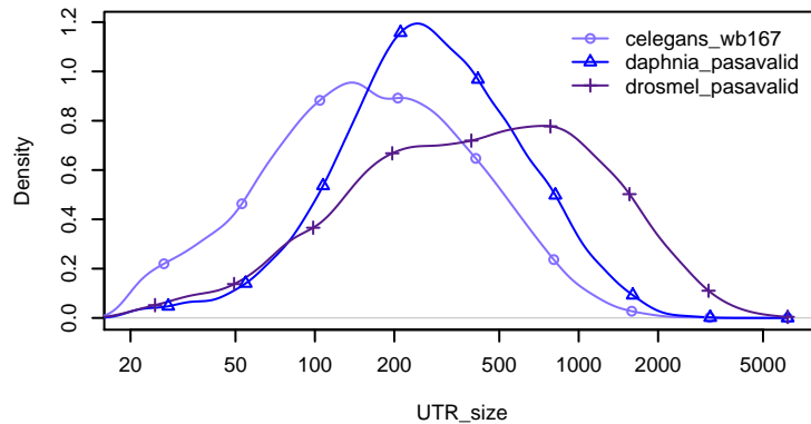
Eukaryote UTR_size
