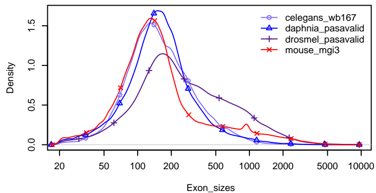
Eukaryote Exon_sizes
